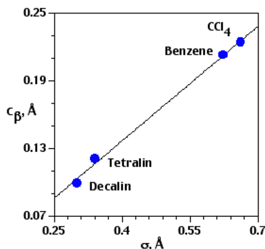
Figure 4. Comparison of the values of c_\beta from ref 46 with our values of \sigma from Table 6.
