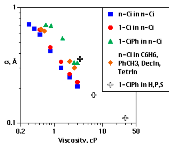
Figure 3. Comparison of the values of \sigma that give the best agreement between experimental and calculated D values and the solvents’ viscosities for n -alkanes in n -alkanes; 1-alkenes in n -alkanes; n -alkanes in benzene, toluene, tetralin, and decalin; 1-phenylalkanes in n -alkanes; and 1-phenylalkanes in HPMN, pristane, and squalane.
