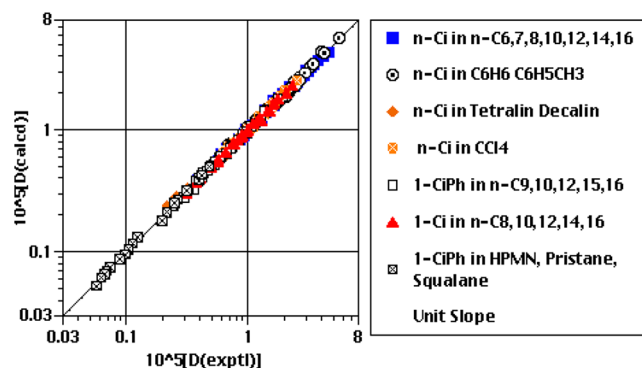
Figure 1. Comparison of the experimental diffusion constants (in \text{cm}^2 \text{ s}^{-1} ) for n -alkane, 1-alkene, and 1-phenylalkane solutes with the predictions of a hydrodynamic bead model based on Kirkwood–Riseman theory.
