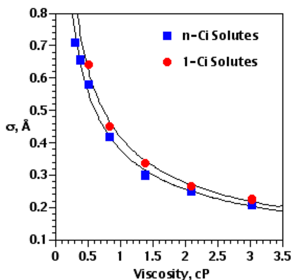
Figure 2. Values of \sigma for the n -alkane and 1-alkene solutes in the n -alkane solvents vs the solvents’ viscosities. The fit is to eq 5.
